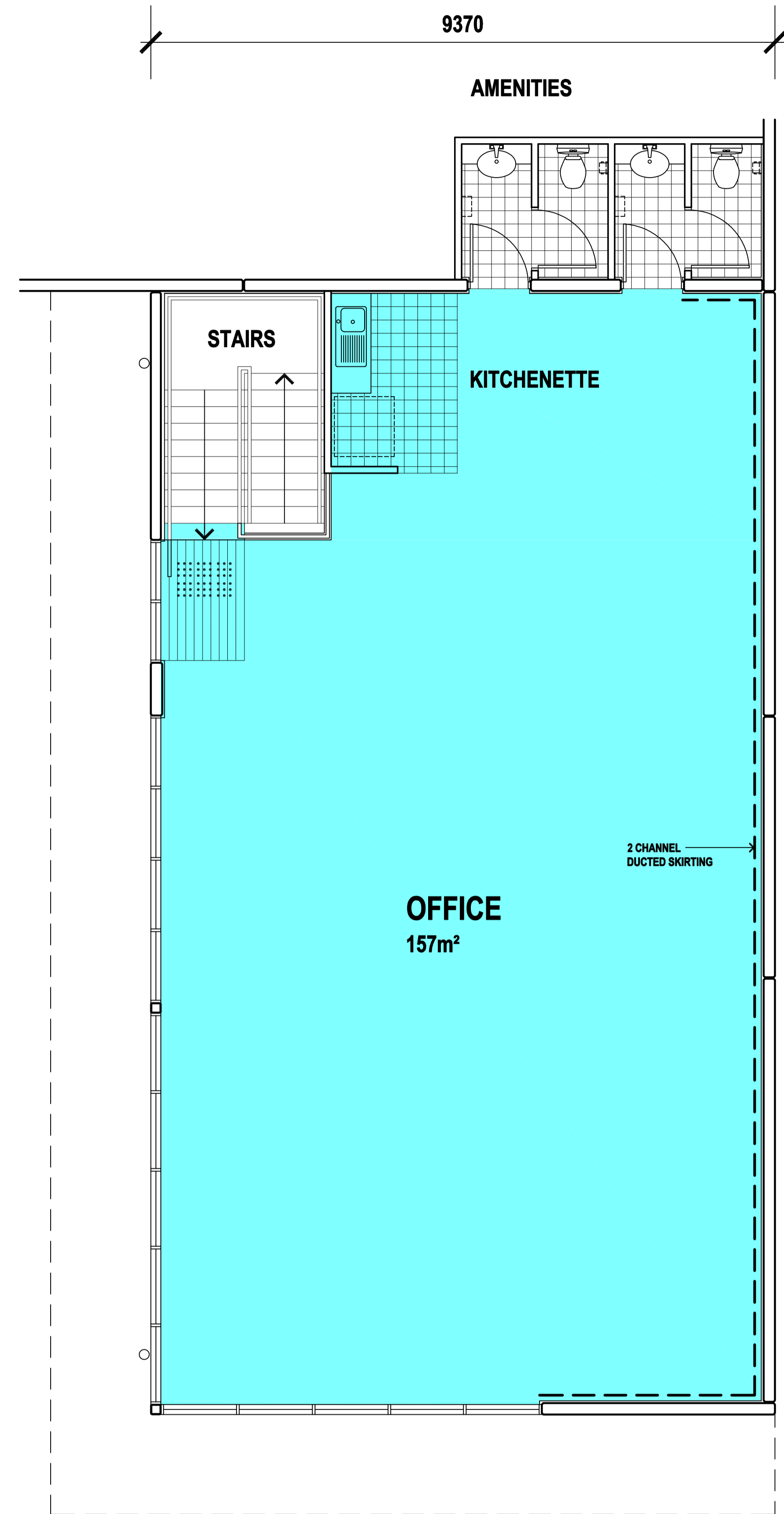
LEVEL 1
